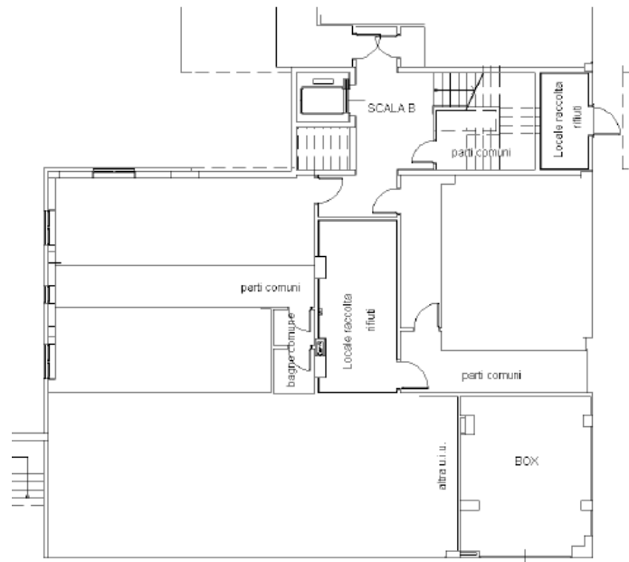
PIANO INTERRATO H=2.40
