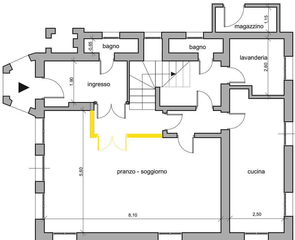
Piano terra
