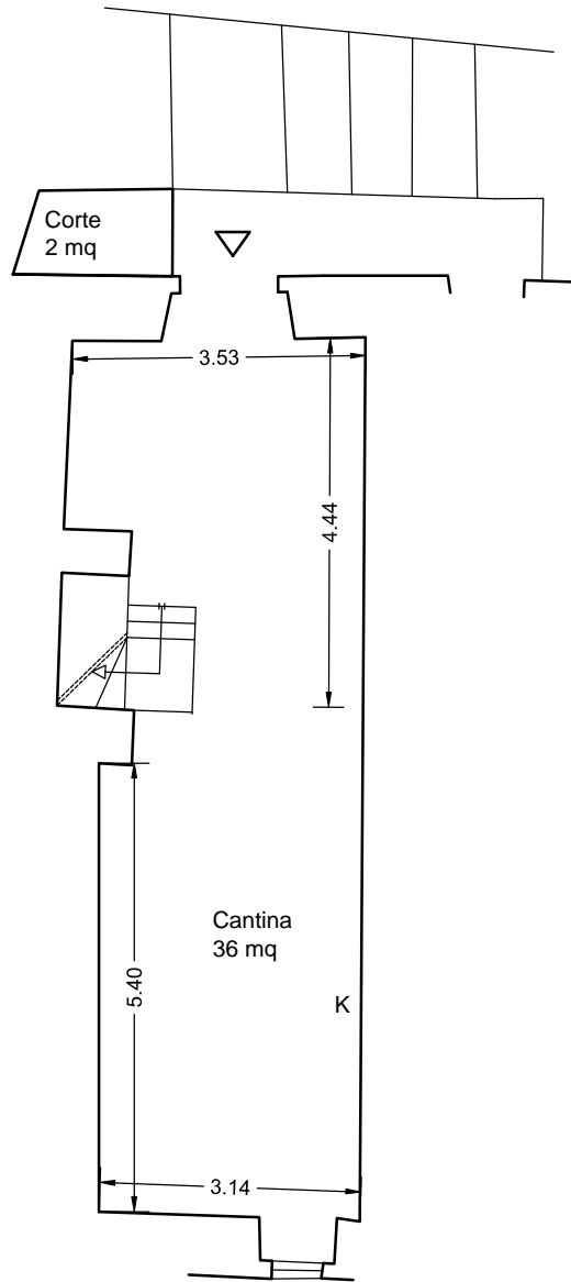
PIANO SEMINTERRATO SCALA 1:100
