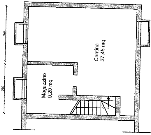
Piano interrato
