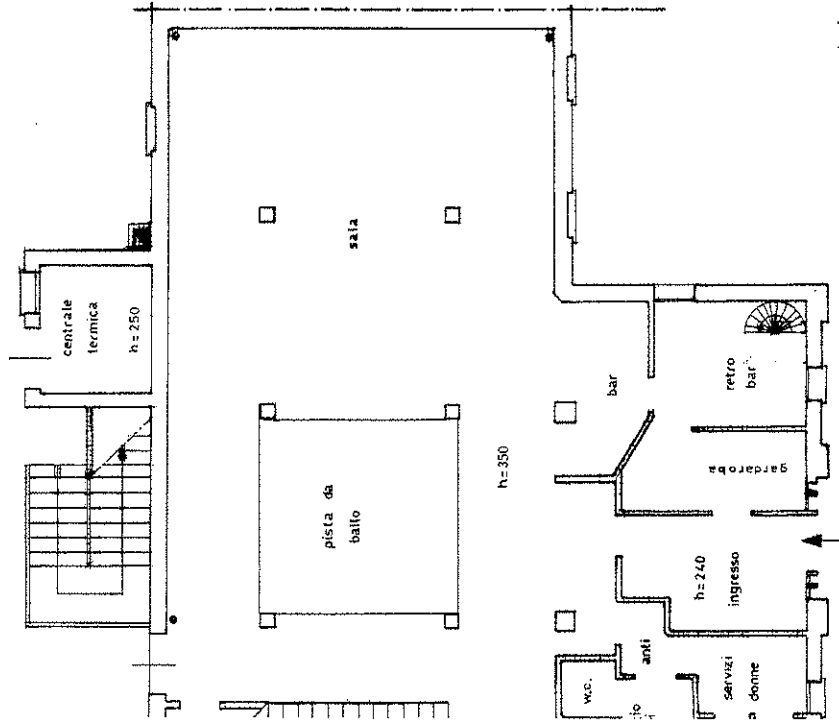
PIANO TERRA
