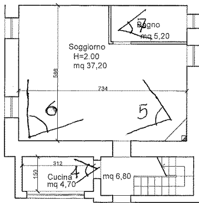
PIANO TERRA
